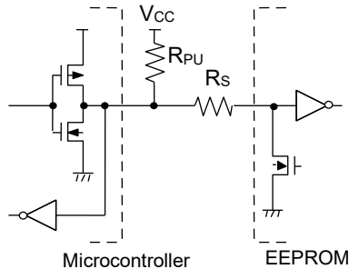
Figure 52. I/O Circuit Diagram
