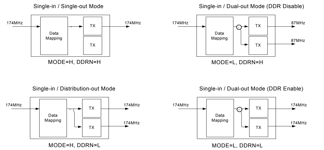
Figure 9. Output Mode Select on MODE,DDRN Pins
