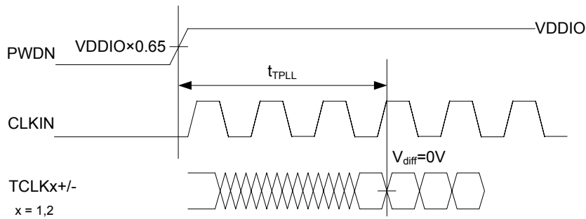
Figure 7. Phase Locked Loop Set Time
