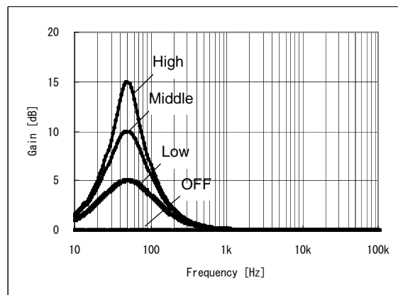
Figure 23. The representative characteristic of Bass Boost
