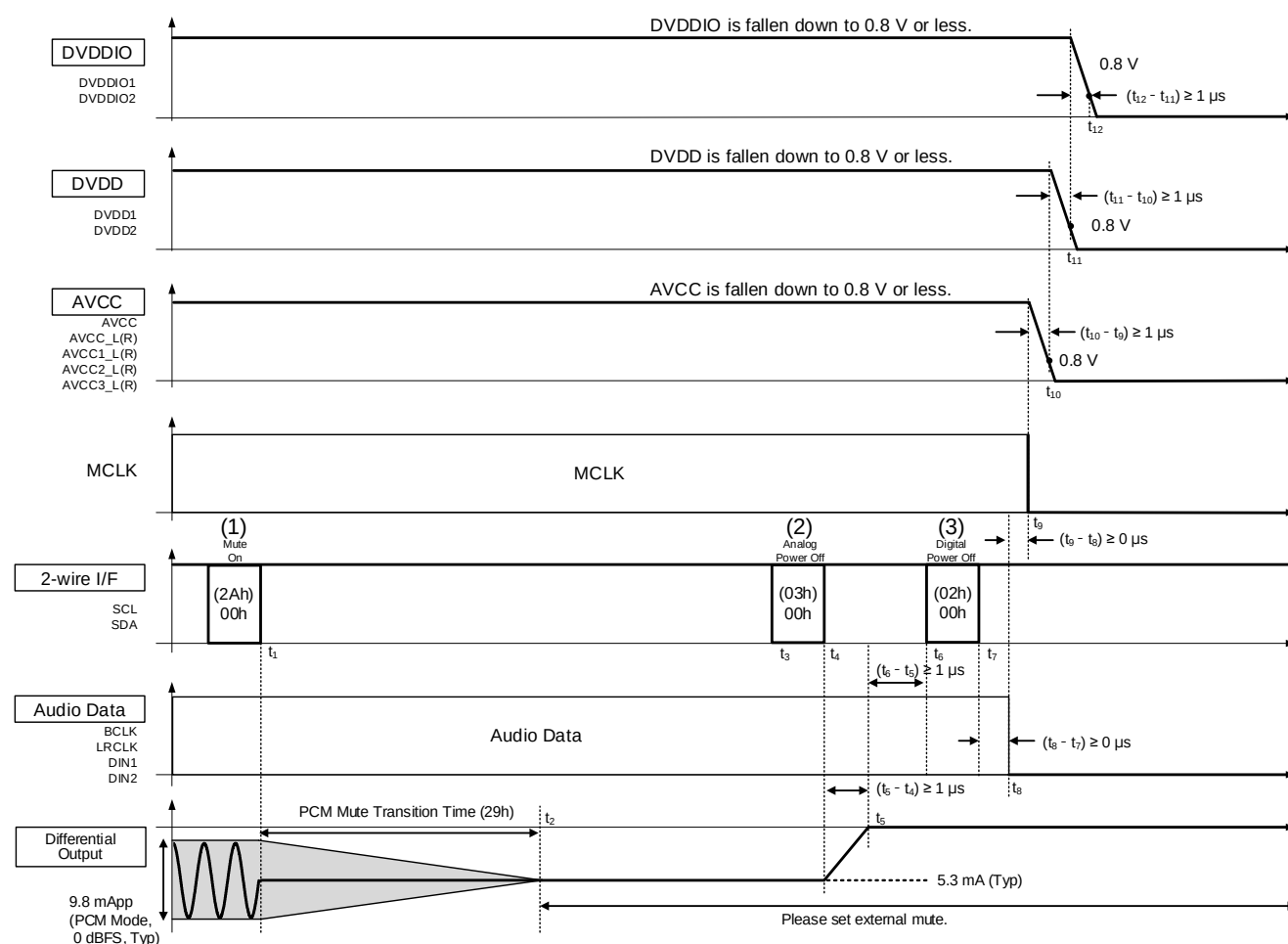
Figure 36. Power-Off Sequence
