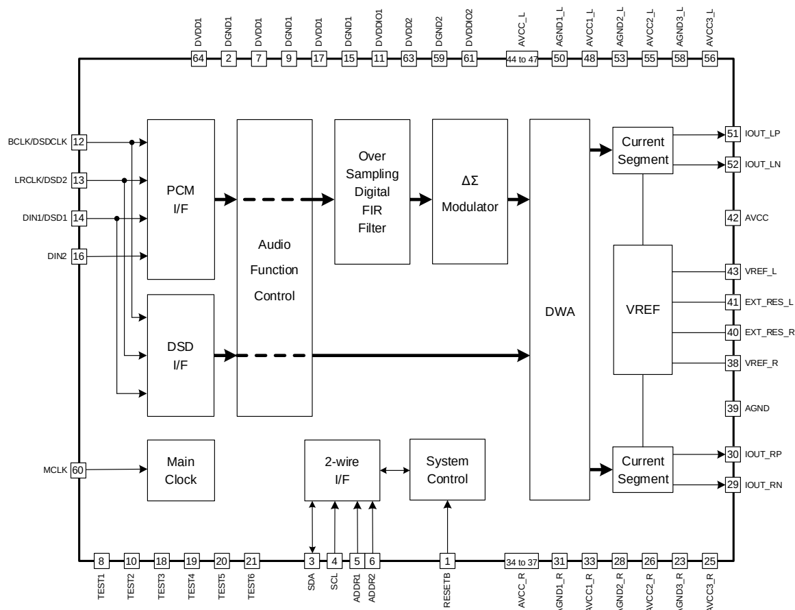
Figure 3. Block Diagram
