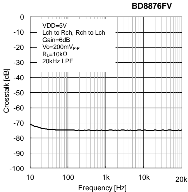
Figure 24. Crosstalk vs. Frequency (BD8876FV, 200mV p-p )
