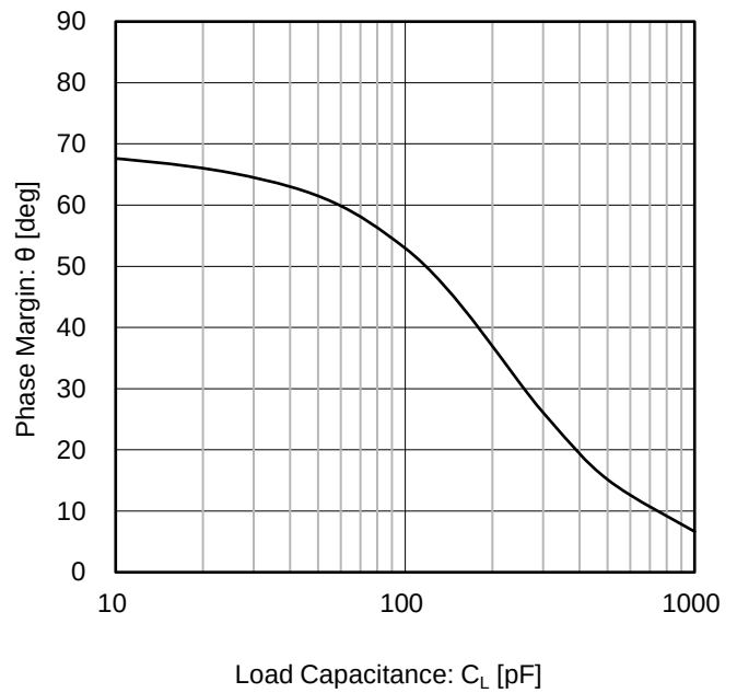
Figure 22. Phase Margin vs Load Capacitance (V S = 5 V, R F = 10 kΩ, G = 40 dB)
