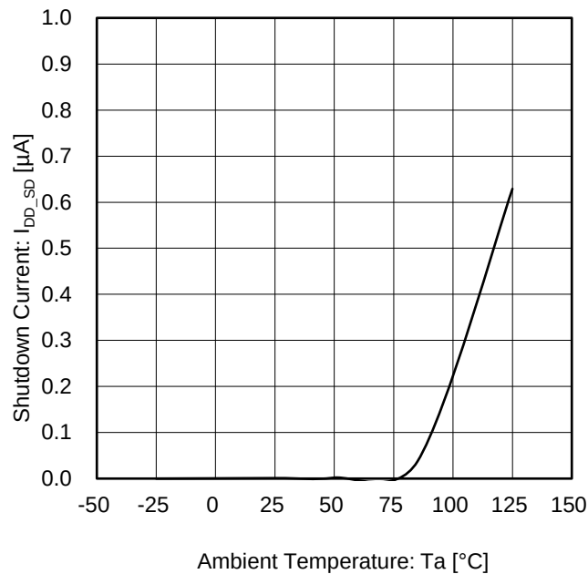
Figure 29. Shutdown Current vs Ambient Temperature (V S = 5 V)
