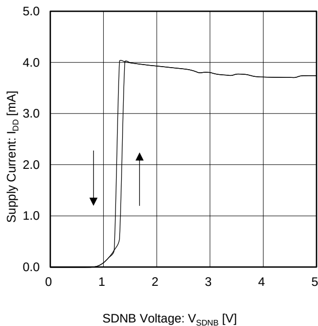
Figure 31. Supply Current vs SDNB Voltage (V S = 5 V, V ICM = 2.5 V, G = 0 dB)
