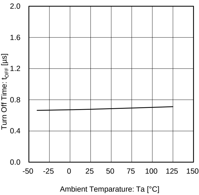
Figure 28. Turn Off Time vs Ambient Temperature ( V_s = 5 V)
