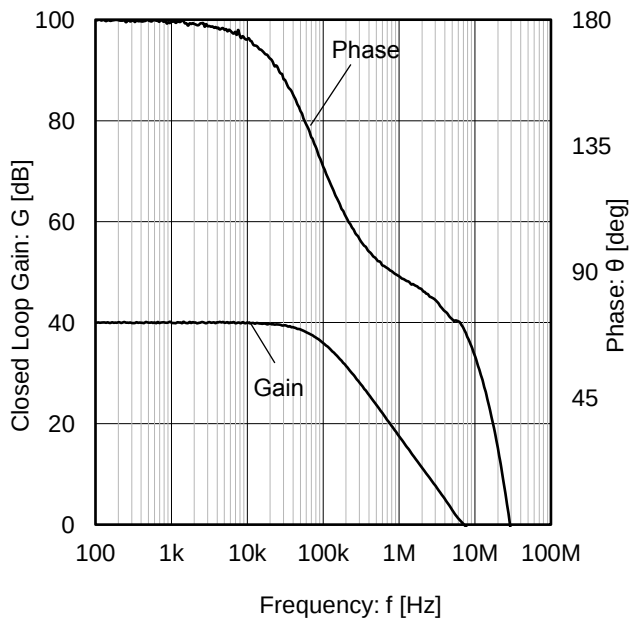
Figure 23. Closed Loop Gain, Phase vs Frequency (V S = 5 V)
