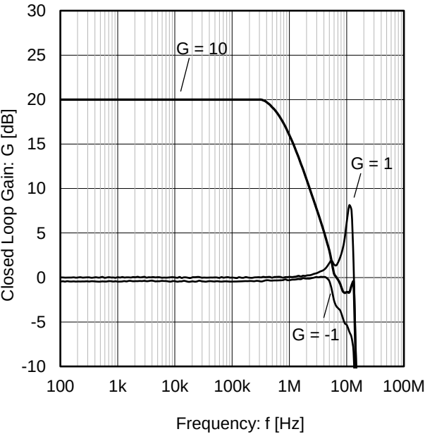
Figure 25. Closed Loop Gain vs Frequency ( V_s = 5 V)
