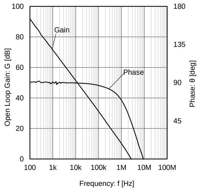
Figure 24. Open Loop Gain, Phase vs Frequency (V S = 5 V)
