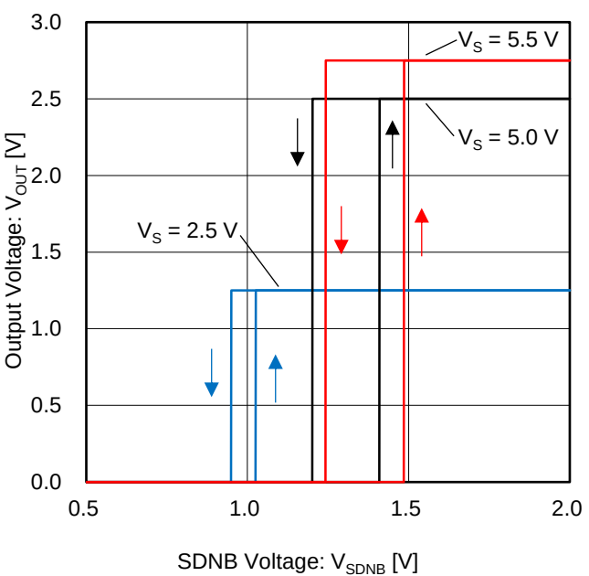
Figure 30. Output Voltage vs SDNB Voltage (V ICM = V S /2, G = 0 dB)
