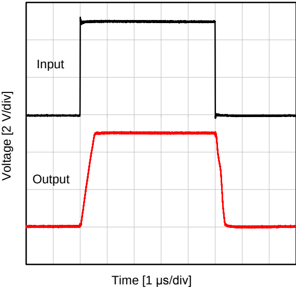
Figure 26. Large-Signal Step Response ( V_s = 5 V, G = 0 dB, R_L = 10 k \Omega , C_L = 100 pF)
