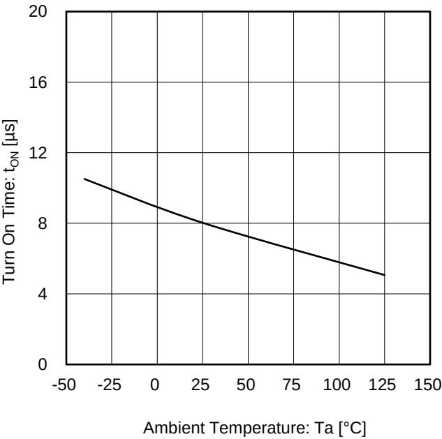
Figure 27. Turn On Time vs Ambient Temperature ( V_s = 5 V)
