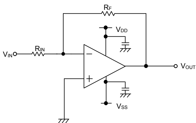
Figure 33. Inverting Amplifier Circuit
