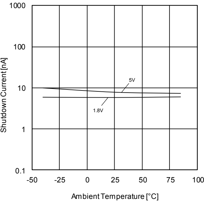
Figure 24. Shutdown Current vs Ambient Temperature (V SHDN =0V)
