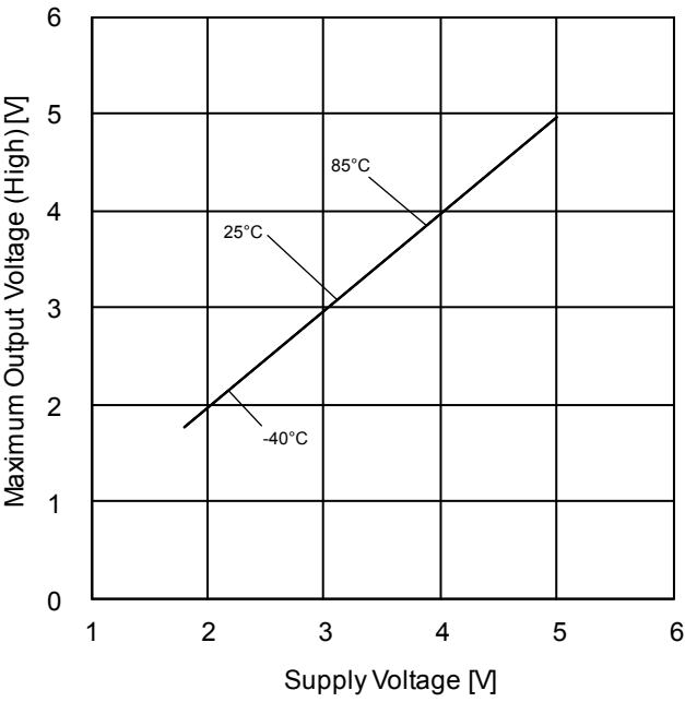
Figure 54. Maximum Output Voltage High vs Supply Voltage ( R_L=2k\Omega )
