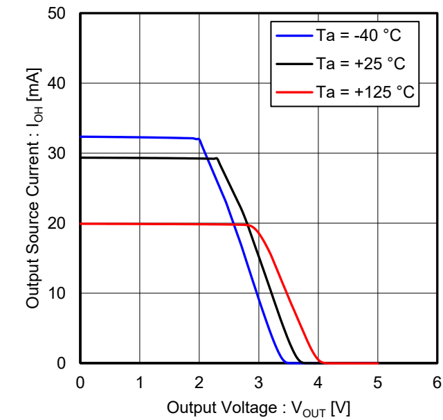
Figure 5. Output Source Current vs Output Voltage (V CC = 5 V)
