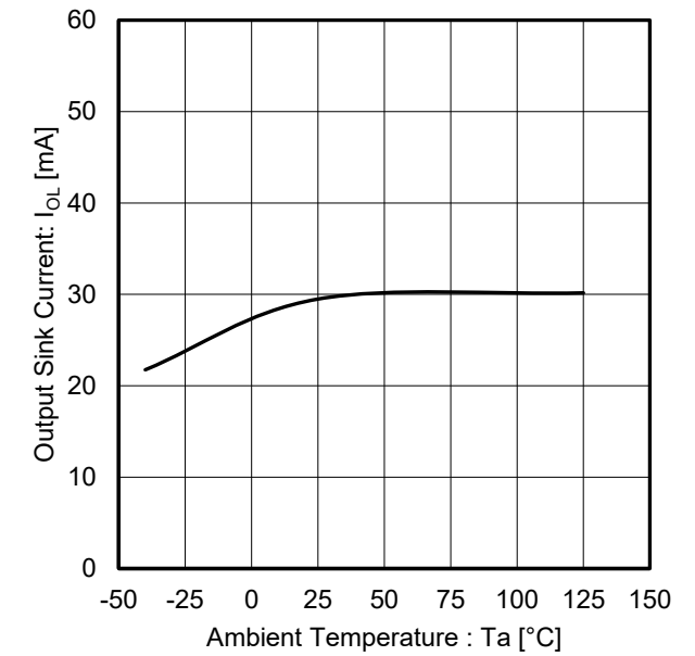
Figure 8. Output Sink Current vs Ambient Temperature (V CC = 5 V, V OUT = 5 V)
