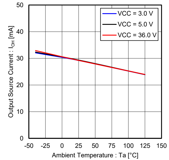
Figure 6. Output Source Current vs Ambient Temperature (V OUT = 0 V)
