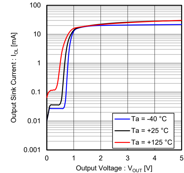
Figure 7. Output Sink Current vs Output Voltage (V CC = 5 V)
