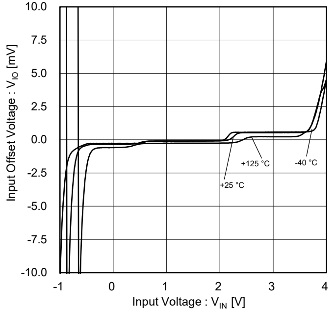
Figure 18. Input Offset Voltage vs Input Voltage (V DD =3.0 V)
