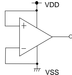
Figure 49. Example of Application Circuit for Unused Comparator
