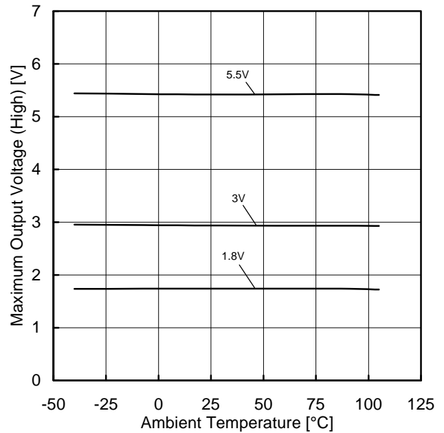
Figure 28. Maximum Output Voltage (High) vs Ambient Temperature ( R_L=10k\Omega )
