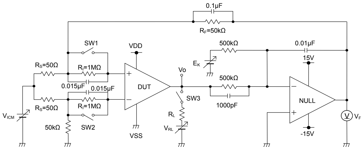
Figure 23. Test Circuit 1
