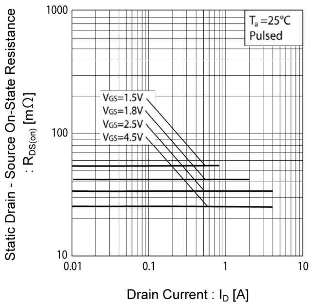
Fig.14 Static Drain - Source On - State Resistance vs. Drain Current ( I_D )
