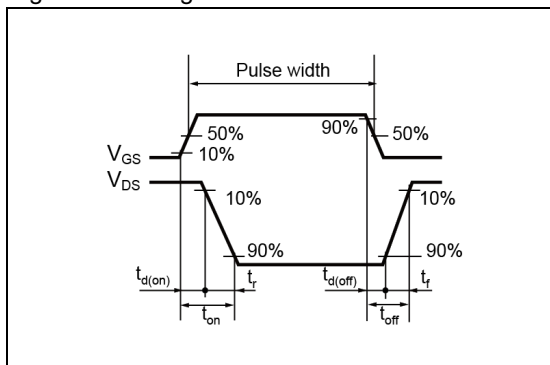
Fig.1-2 Switching Waveforms
