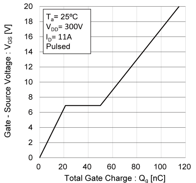
Fig.16 Gate charge
