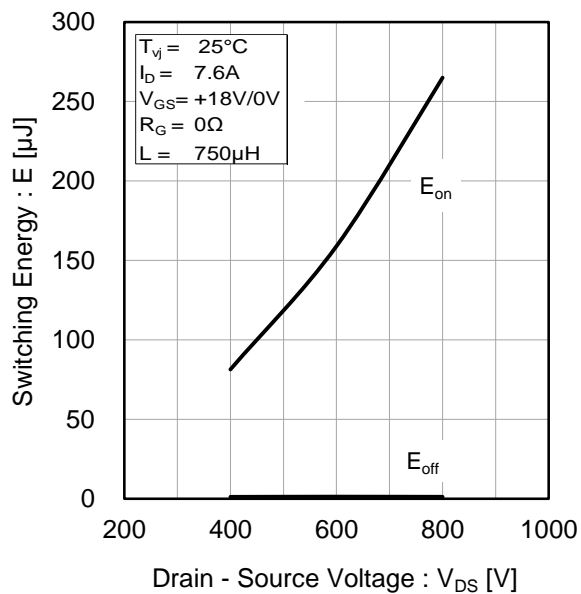
Fig.20 Typical Switching Loss vs. Drain - Source Voltage
