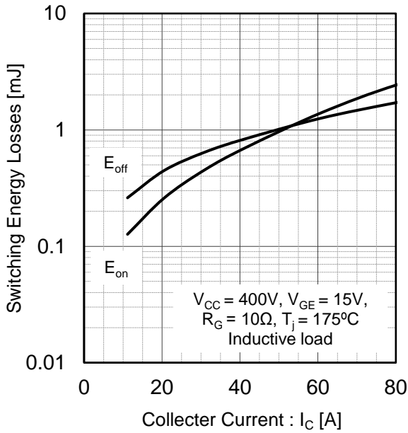
Fig.13 Typical Switching Energy Losses vs. Collector Current
