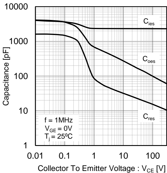
Fig.15 Typical Capacitance vs. Collector Emitter to Voltage
