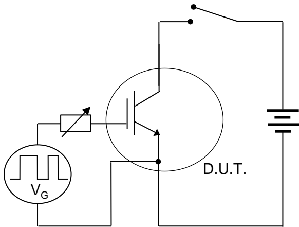
Fig.24 Short Circuit
