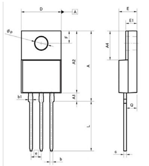
TO-220FN, (TO-220FN)
