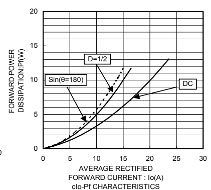
c_{\theta} - P CHARACTERISTICS
