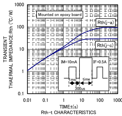
Rth-t CHARACTERISTICS
