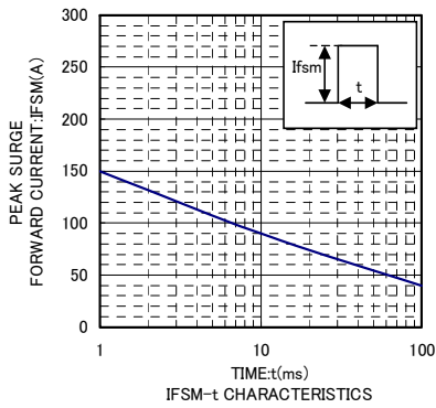
IFSM-t CHARACTERISTICS
