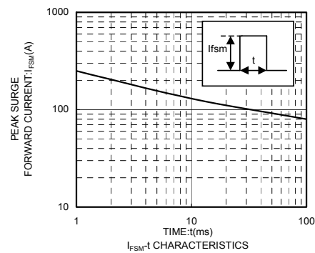
I_{FSM}-t CHARACTERISTICS
