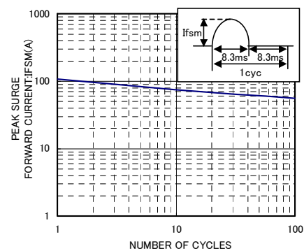
IFSM-CYCLE CHARACTERISTICS
