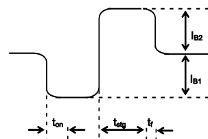
BASE CURRENT WAVEFORM
