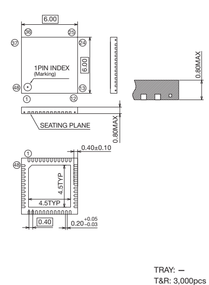
P-WQFN48-0606-0.40-T63-MC
