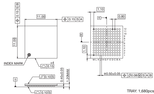
P-TFBGA144-1111-0.80-1
