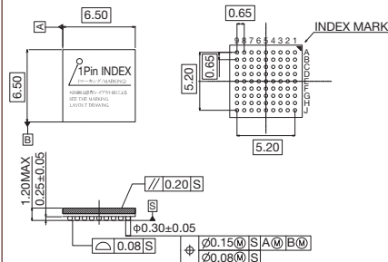
P-TFBGA81-6.5x6.5-0.65-9-MC
