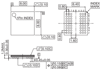
P-TFBGA54-0808-0.80-9
