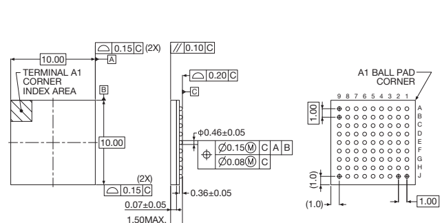
P-LBGA81-1010-1.00-1-MC
