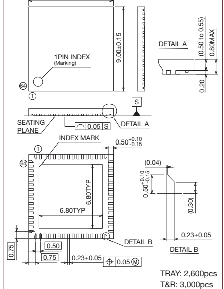
P-WQFN64-0909-0.50-63
