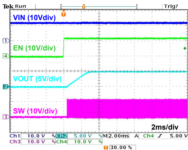
Figure 12. Rise-up Waveform (V EN =0V→12V, I OUT =3A)
