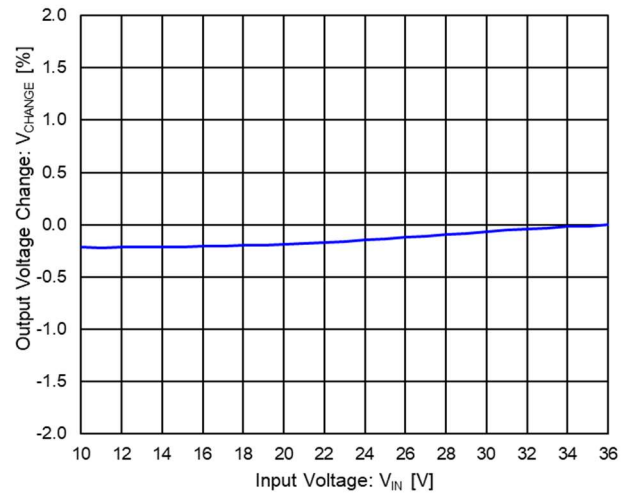
Figure 11. V OUT Line Regulation (V OUT =5V, I OUT =3A)
