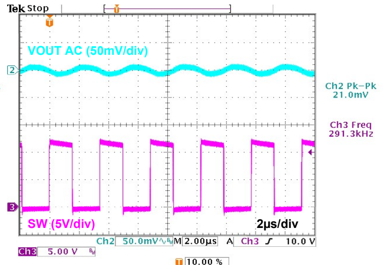
Figure 15. SW Waveform (VIN=12V, VOUT=5V, IOUT=3A)
