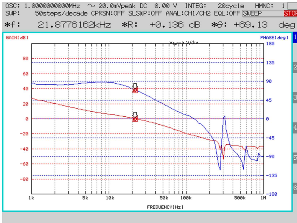
Figure 16. Frequency Response (VIN=12V, VOUT=5V, IOUT=3A)
