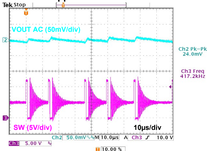
Figure 14. SW Waveform (VIN=12V, VOUT=5V, IOUT=30mA)
