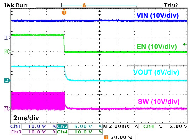
Figure 13. Shut-down Waveform (V EN =12V→0V, I OUT =3A)
