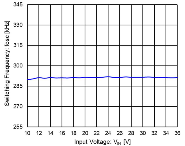
Figure 8. Switching Frequency vs Input Voltage ( V_{OUT}=5V , I_{OUT}=3A )
