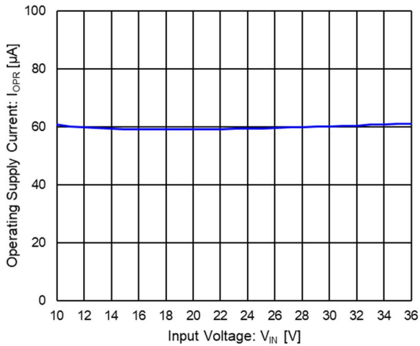
Figure 7. Operating Quiescent Current vs Input Voltage ( V_{IN}=12V , V_{OUT}=5V , I_{OUT}=0A )
