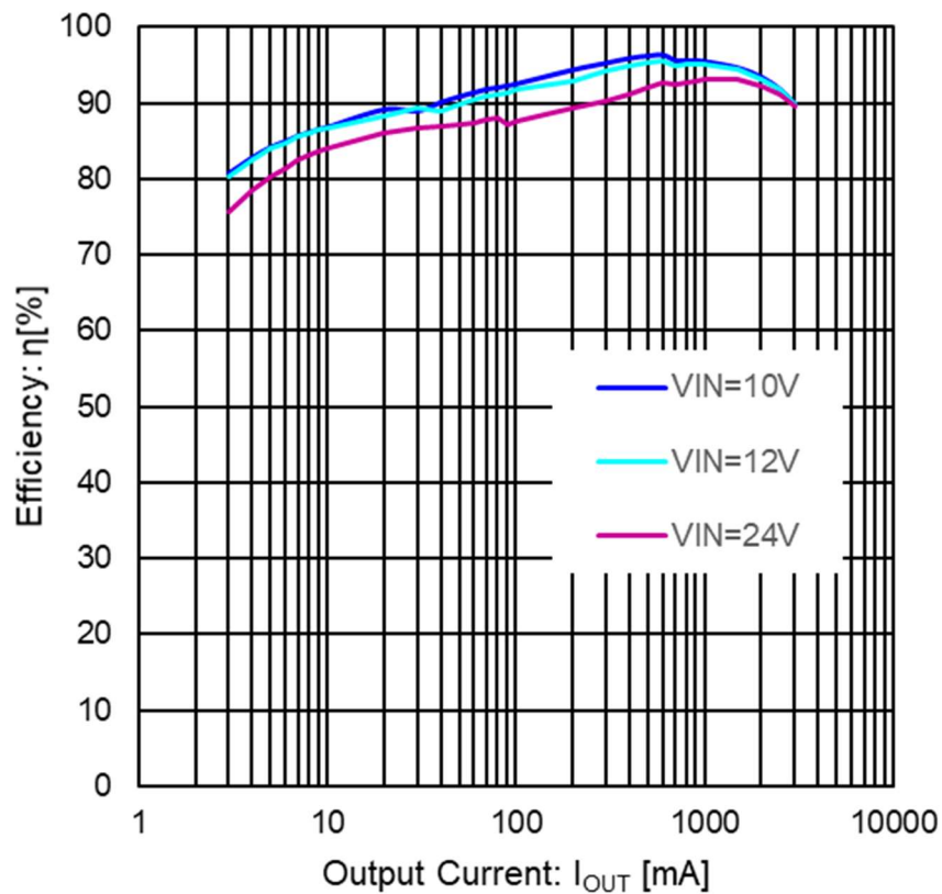
Figure 9. Efficiency vs Output Current ( V_{OUT}=5V )
