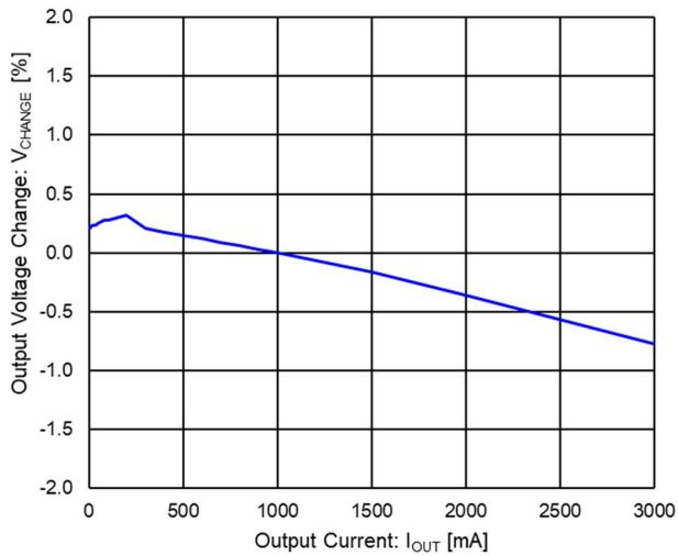
Figure 10. V OUT Load Regulation (V IN =12V, V OUT =5V)
