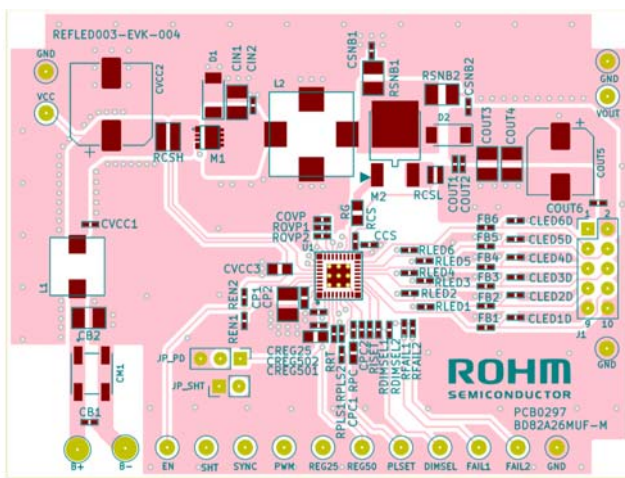
Figure 7. Top layer layout (Top view)
