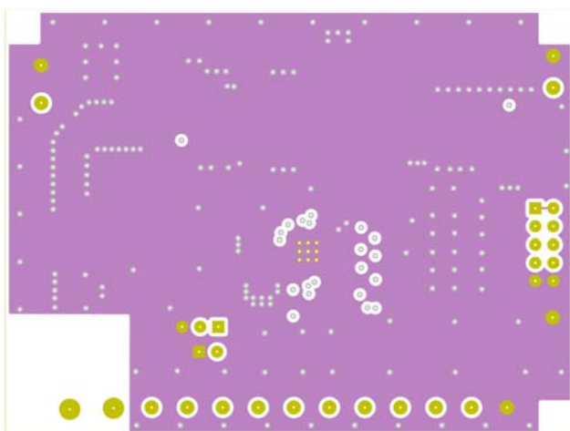
Figure 9. 3rd layer layout (Top view)
