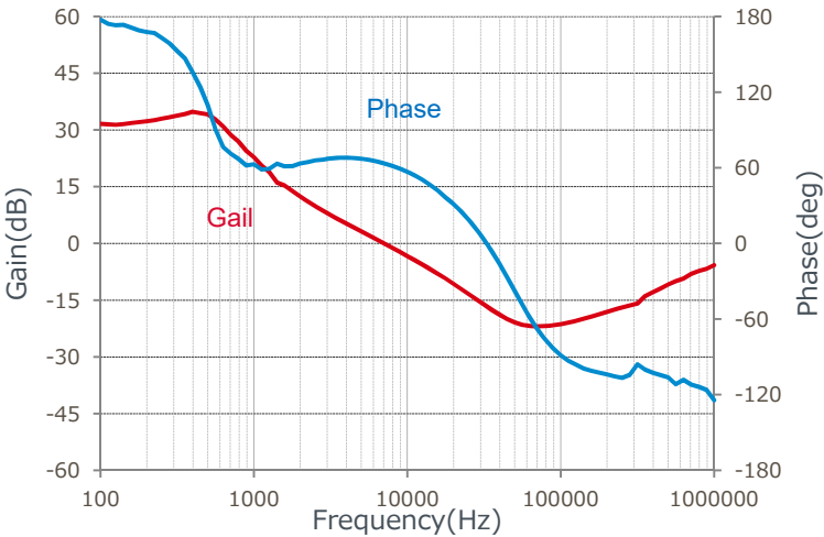
Figure 12. Gain, Phase vs Frequency (VCC=13.5V)
