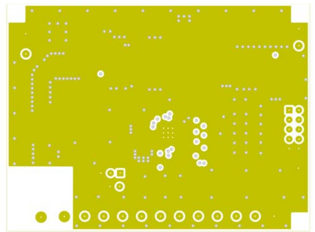
Figure 8. 2nd layer layout (Top view)
