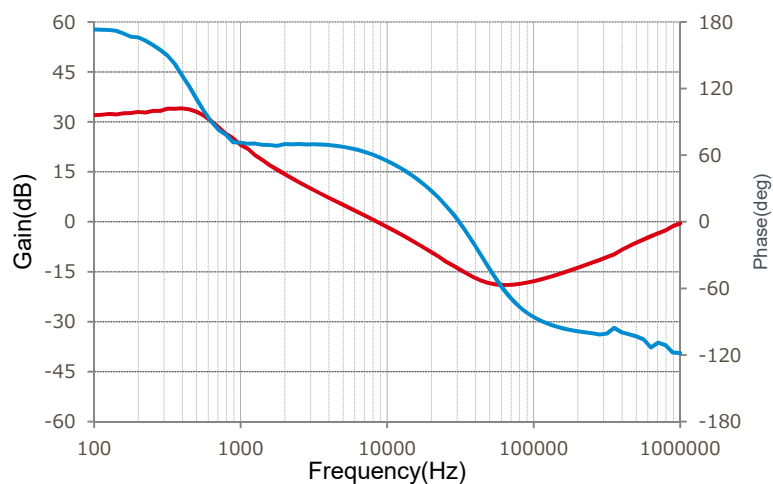
Figure 12. Gain, Phase vs Frequency (VCC=13.5V)
