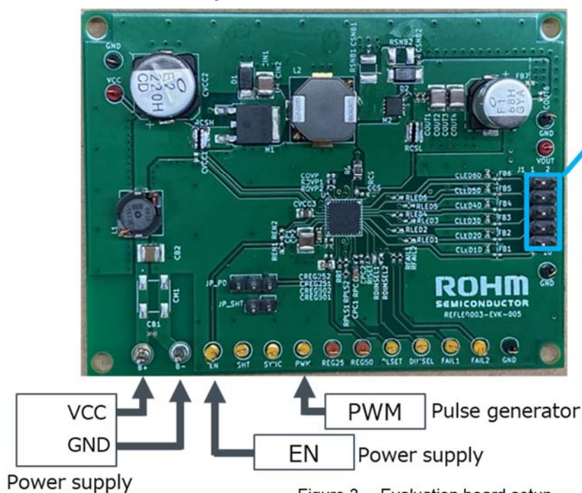
Figure 3. Evaluation board setup
