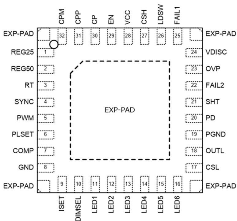
Figure 5. Pin configuration
