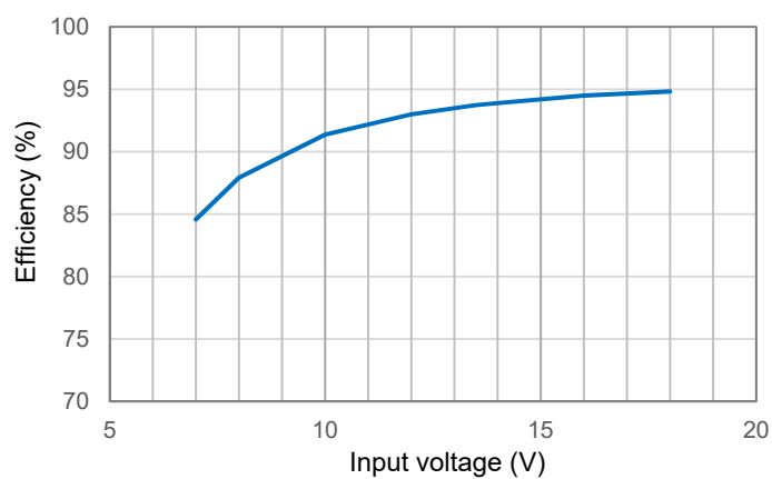
Figure 11. Efficiency vs Input voltage
