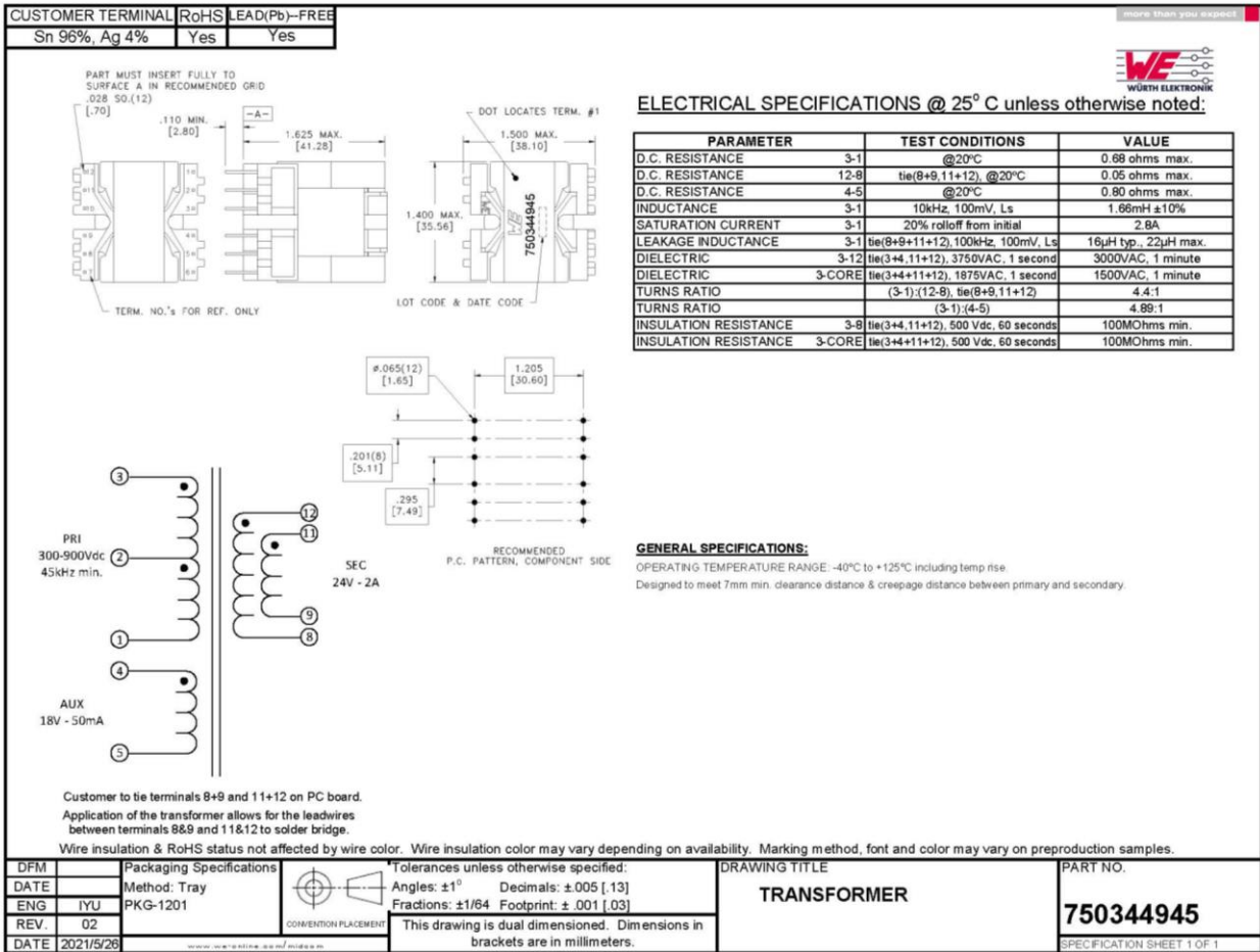
Figure 5. Transformer Specification
