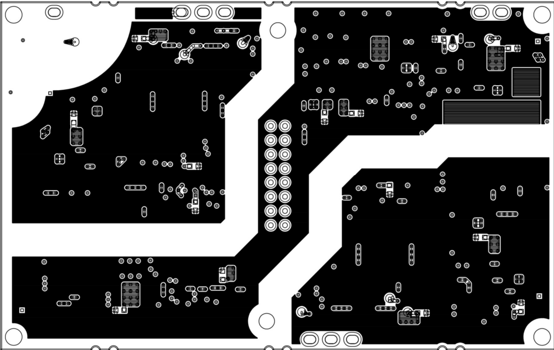
Figure 29. Bottom-Layer (Top view)
