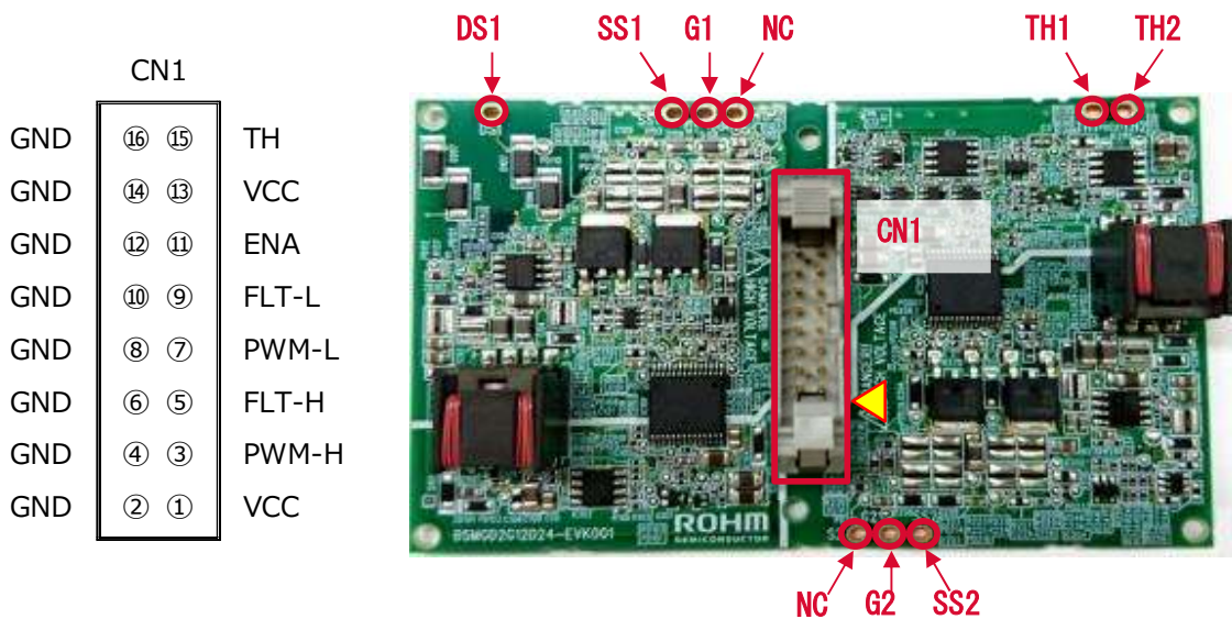
Figure 2. Pin assignment
