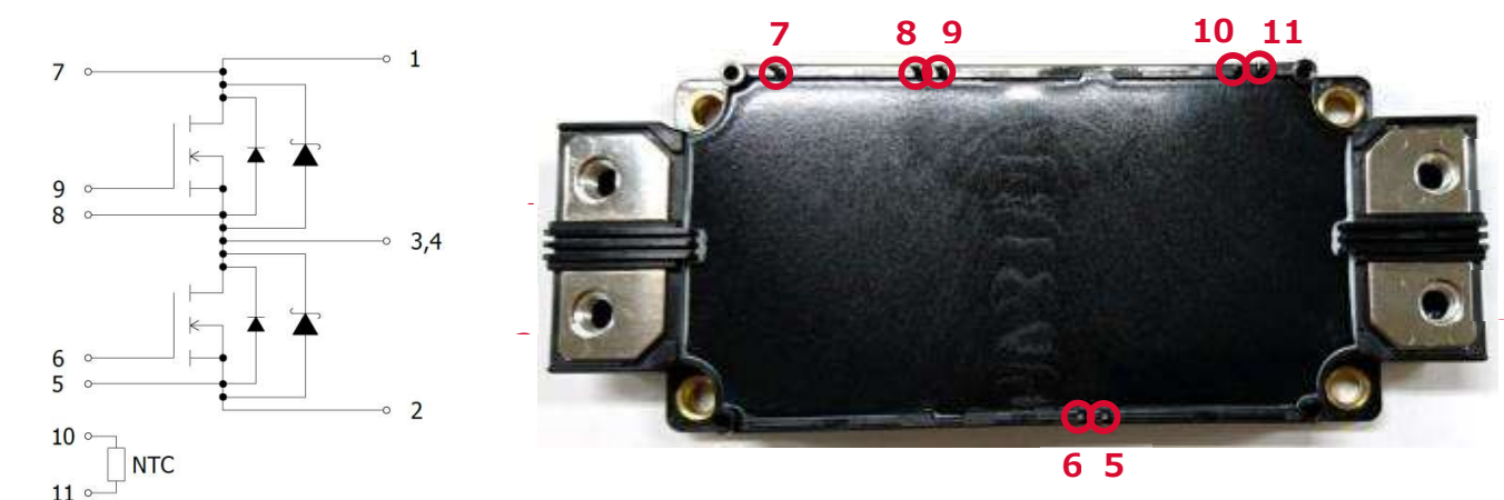
Figure 18. SiC module’s pins numbering
